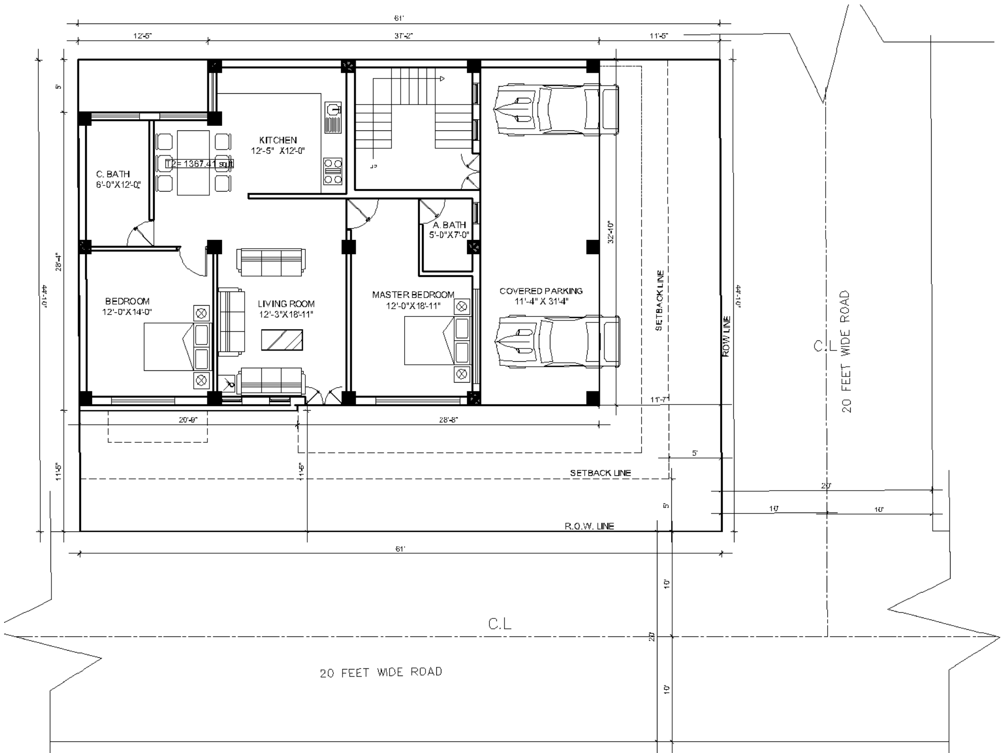
SITE PLAN
